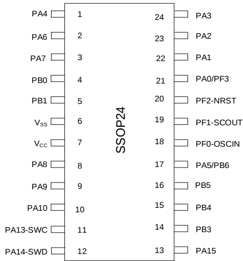
图 3-1 SSOP24 Pinout1 PY32M030E1xM7 (Top View)
